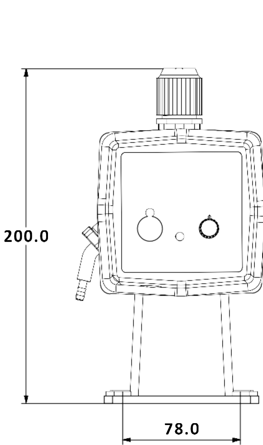
FRONT VIEW
