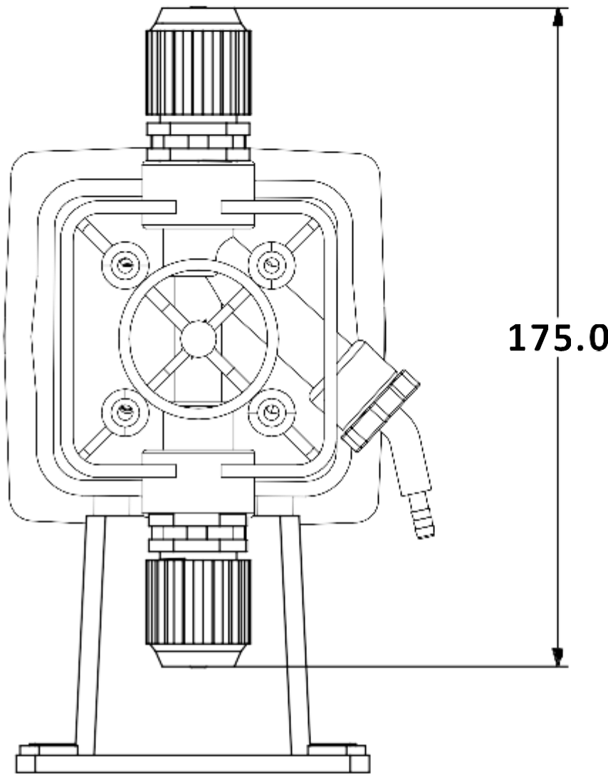
BACK VIEW
