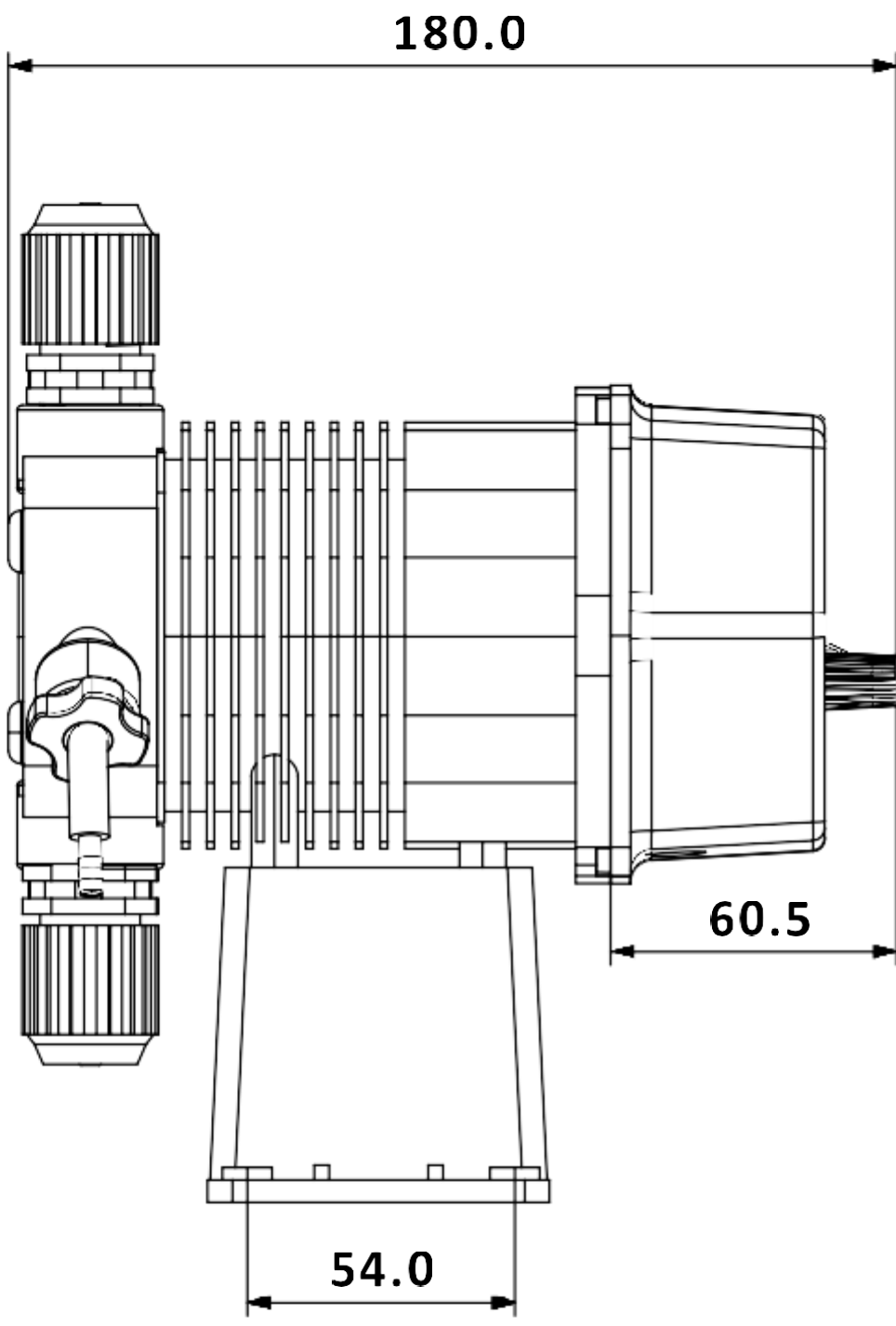
LEFT HAND SIDE VIEW
