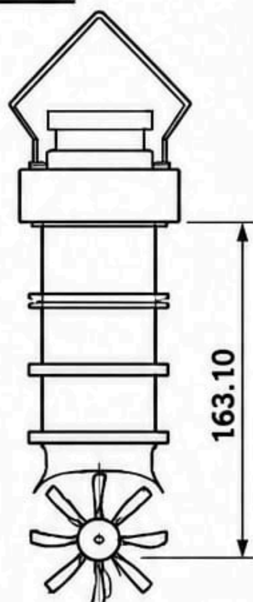
Extra Long Insertion Sensor (150NB)
