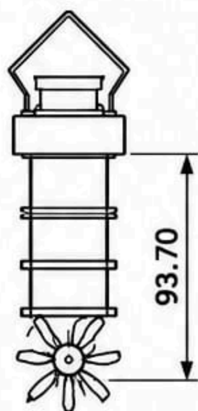
Regular Insertion Sensor (40NB, 50NB, 65NB, 80NB)
