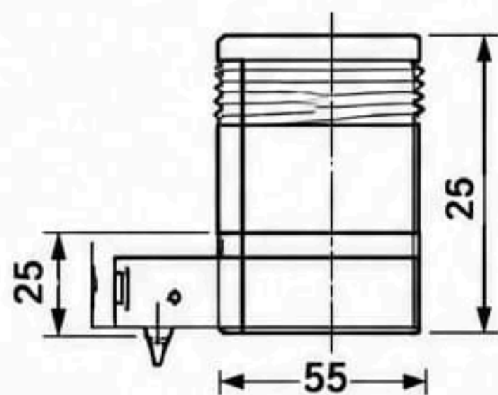
SS Weldon Adaptor
