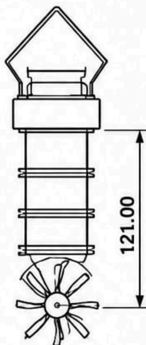
Long Insertion Sensor (100NB, 125NB)
