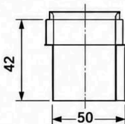
Small pvc adaptor
