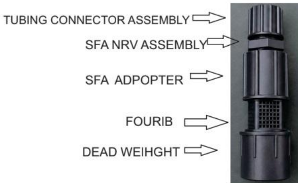
SUCTION FILTER VALVE ASSEMBLY
