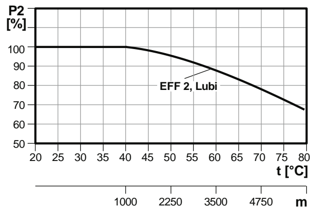
Fig. 4 Relationship between motor output (P 2 ) and ambient temperature
