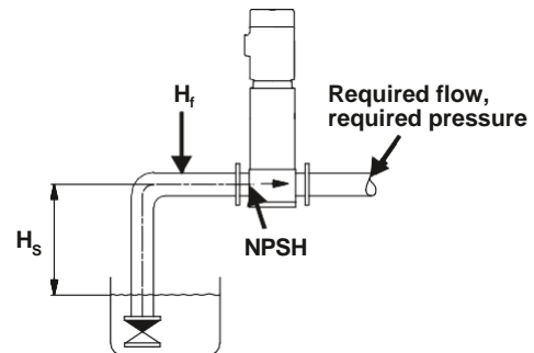
Fig. 9 Dimensional data
