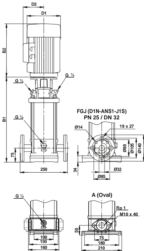
Dimensions & Weights of LCR1, LCRN Pump
