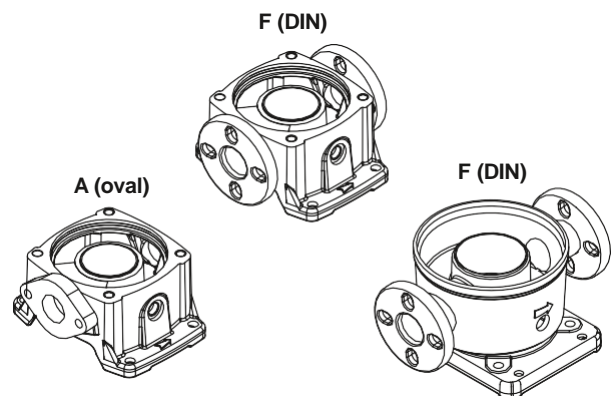
Fig. 11 Pump connections
