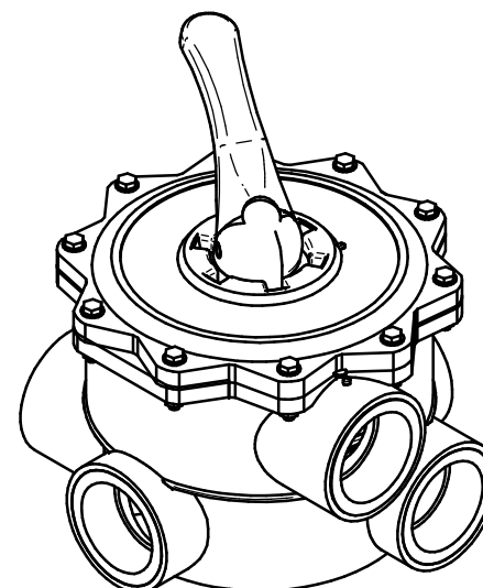
50nb SIDE MOUNT FILTER MULTIPORT VALVE (DIRECT BODY THREADING MIDAS TYPE) GENERAL ASSEMBLY
