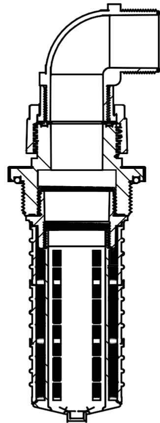
SECTION E-E
