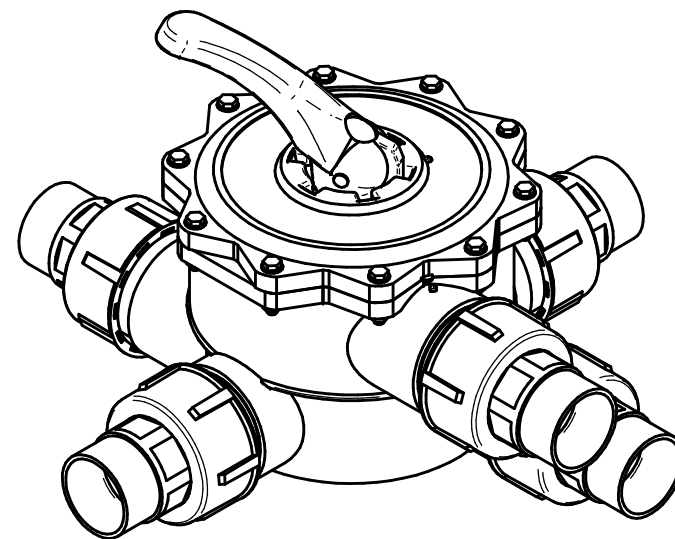
50nb SIDE MOUNT FILTER MULTIPORT VALVE (UNION TYPE) GENERAL ASSEMBLY
